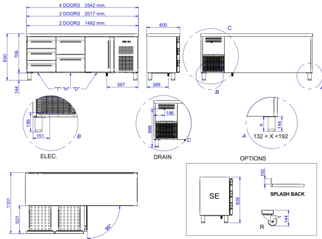
DRAWER DIMENSIONS
