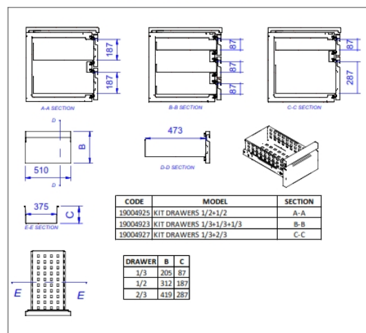
DRAWER DIMENSIONS
